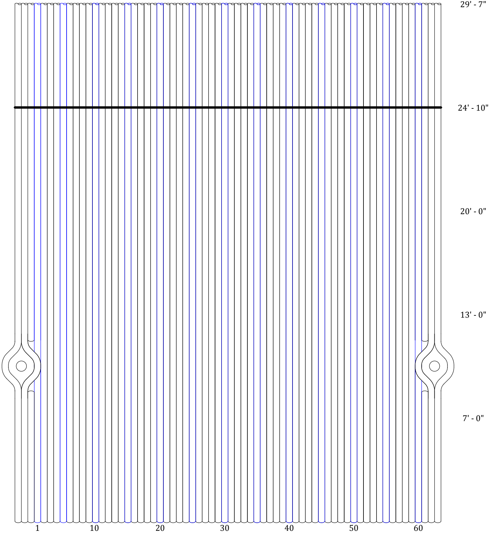
WEST WALL 2.5 O.D. x 0.165 MWT - SA-178 CARBON STEEL
