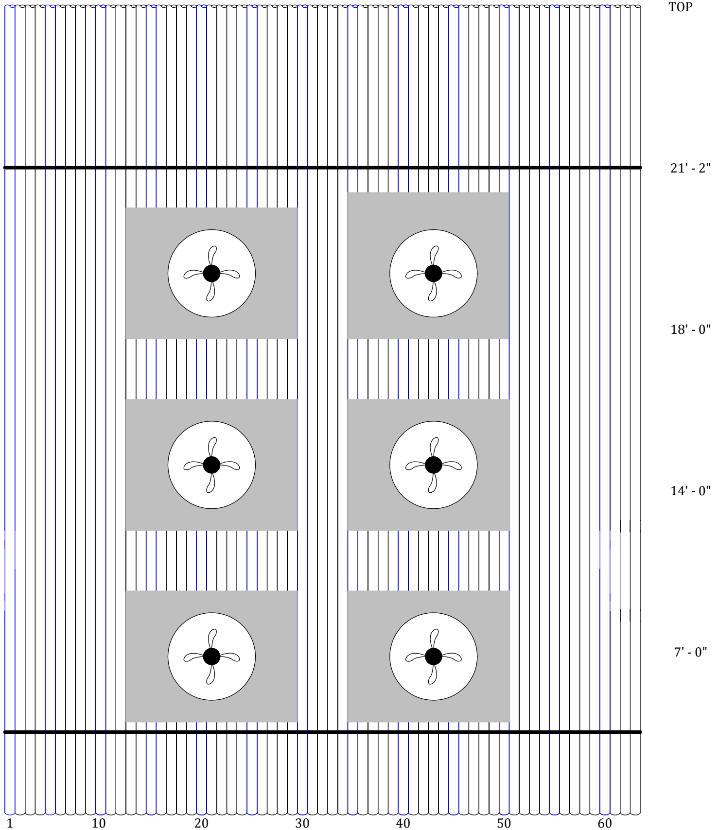
EAST WALL 2.5 O.D. x 0.165 MWT - SA-178 CARBON STEEL
